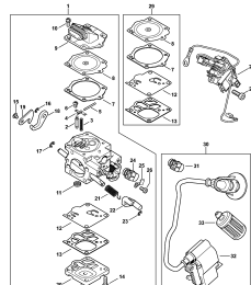
Carburetor WJ-134
