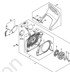
Rewind starter, Hand guard
