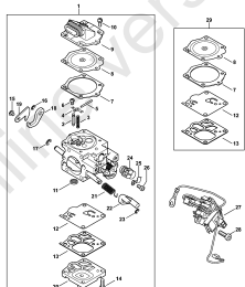
Carburetor WJ-140
