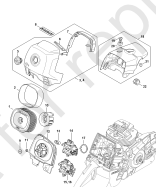
Ignition system
