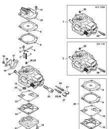
Carburetor WJ-135
