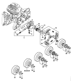
Oil pump, Clutch
