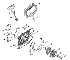
Rewind starter
