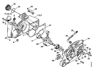
Crankcase, Crankshaft
