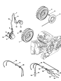
Ignition system, Wiring harness
