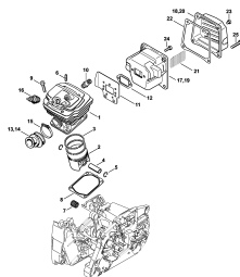
Cylinder, Muffler
