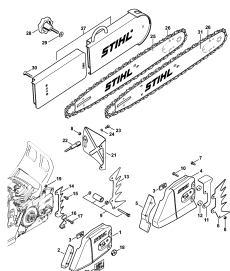
Chain sprocket cover, Guide bar
