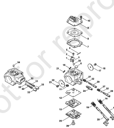
Carburetor HD-50, HD-51
