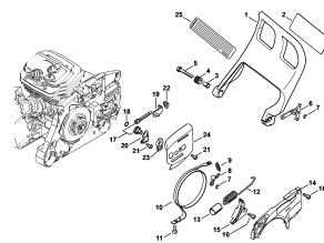
Hand guard, Chain brake, Chain tensioner
