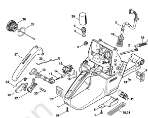
Tank housing
