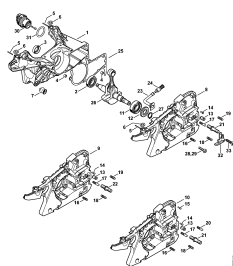
Crankcase
