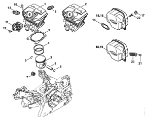
Cylinder, Muffler
