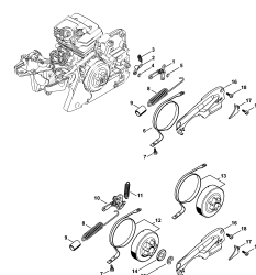
Chain brake
