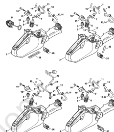
Tank housing
