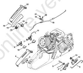
Throttle control
