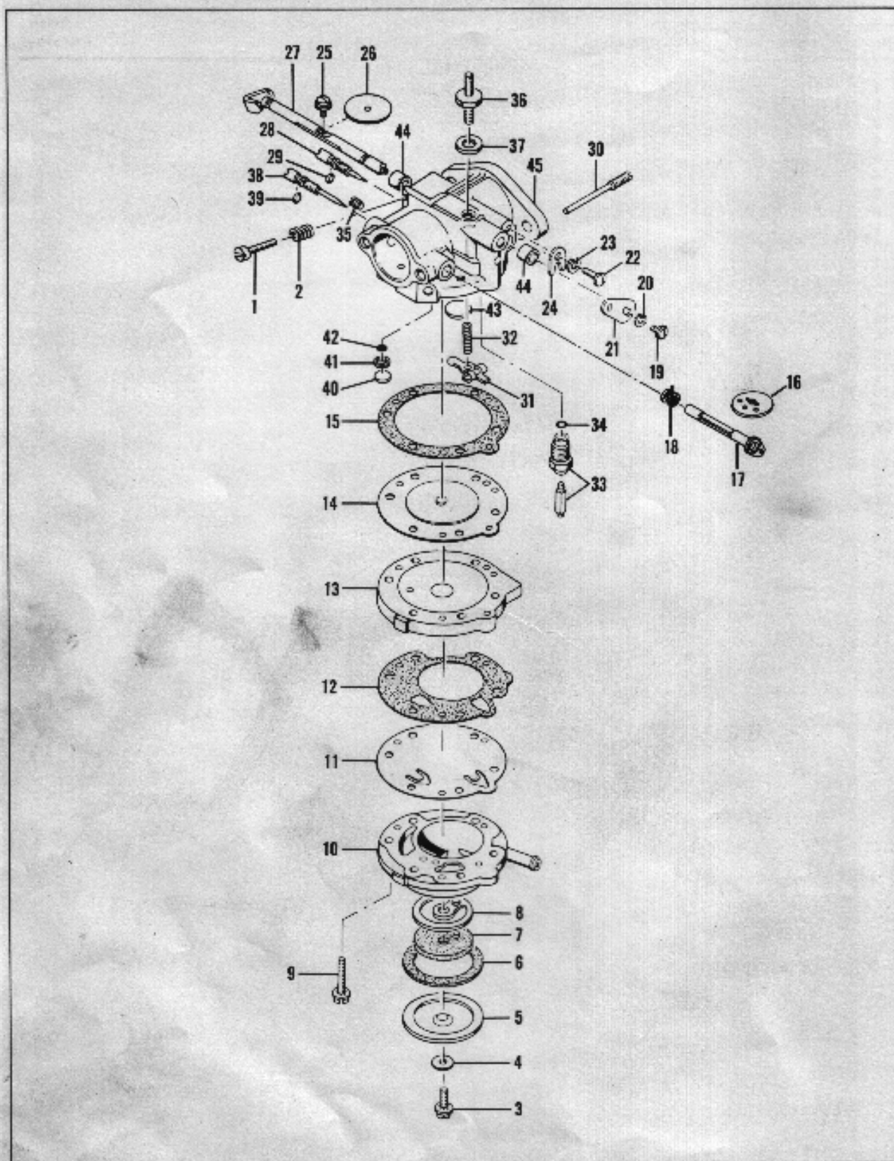
Figure 5. Carburetor
