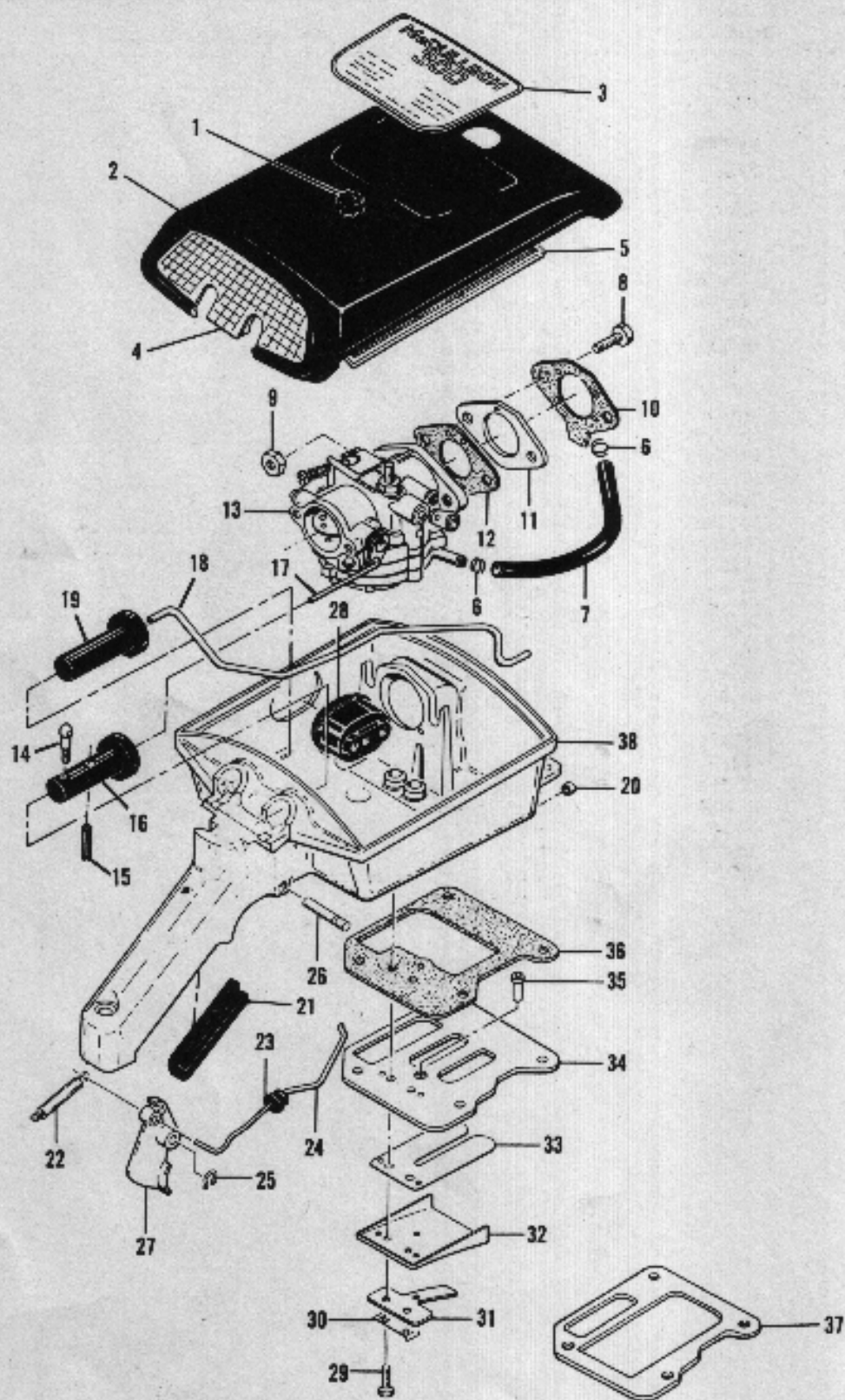
Figure 4. Cover and Airbox Assemblies
