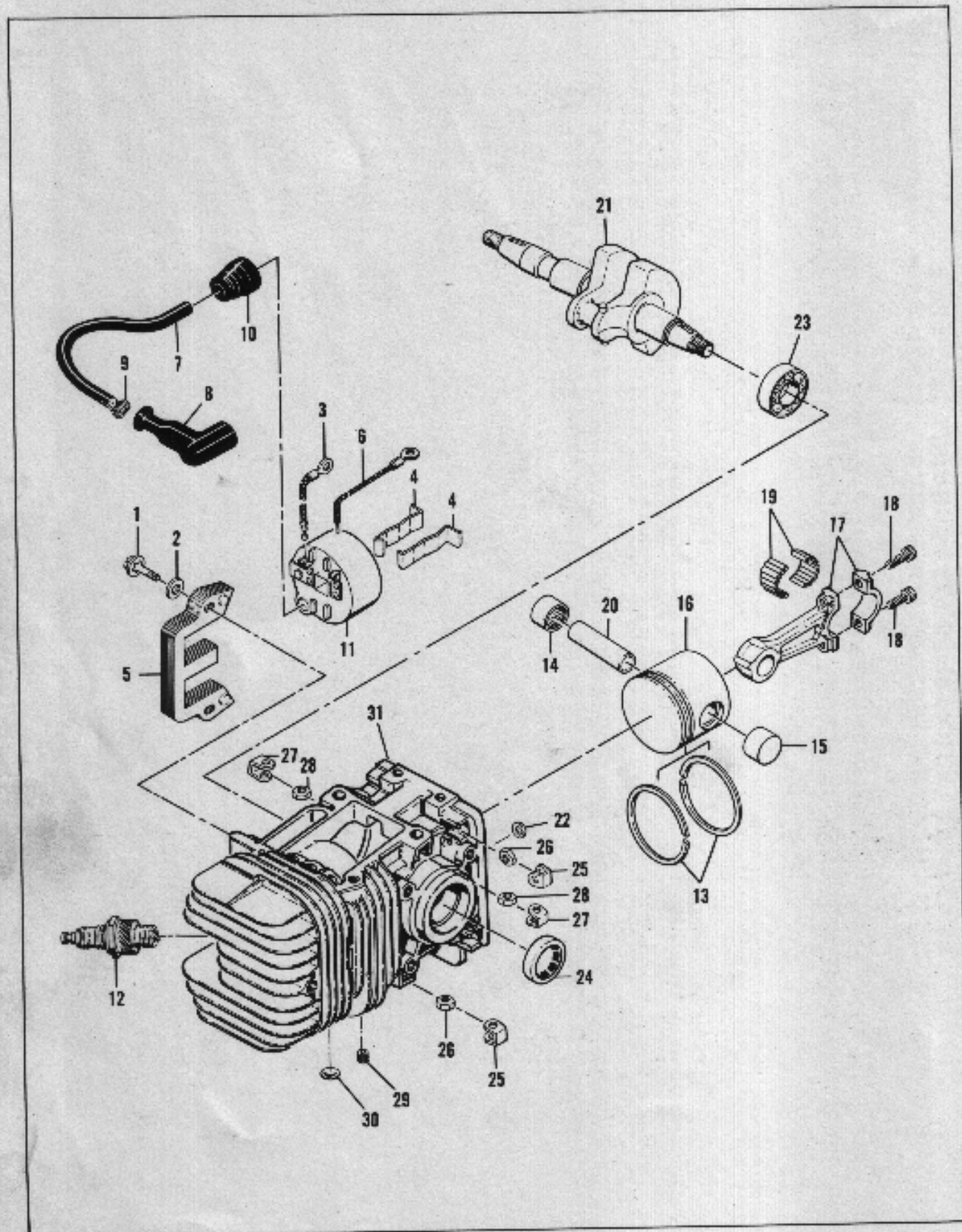
Figure 6. Powerhead Assembly
