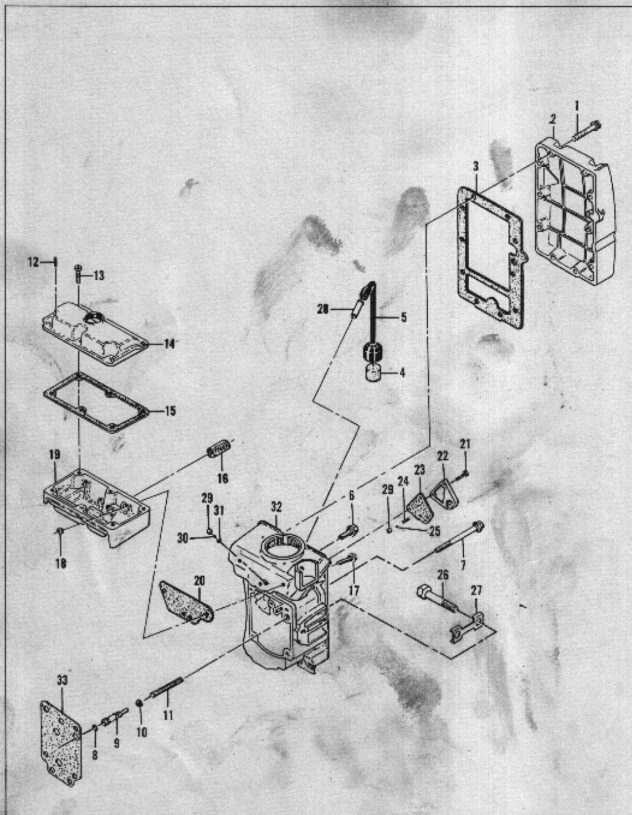
Figure 3. Oiler Tank and Fuel Tank Assemblies
